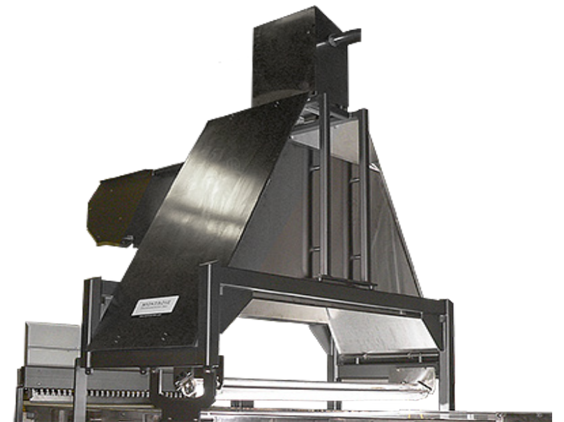
MT-60 In-line Inspection Systems for Toaster Pastries
